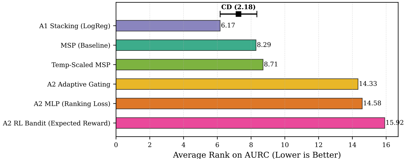
Friedman Mean Ranks (Nemenyi CD = 2.18, N=12, k=6)
