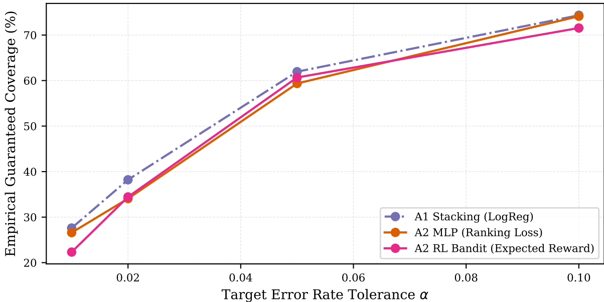
Conformal Prediction Finite-Sample Coverage Guarantees
