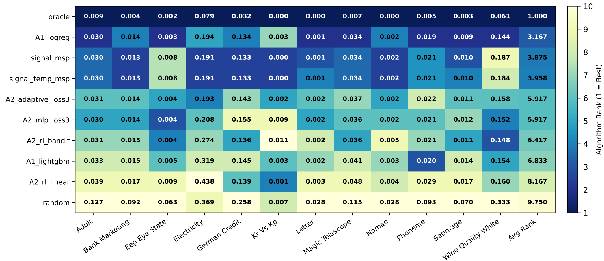
Cross-Dataset AURC Performance Matrix (Tiers: ABC)
