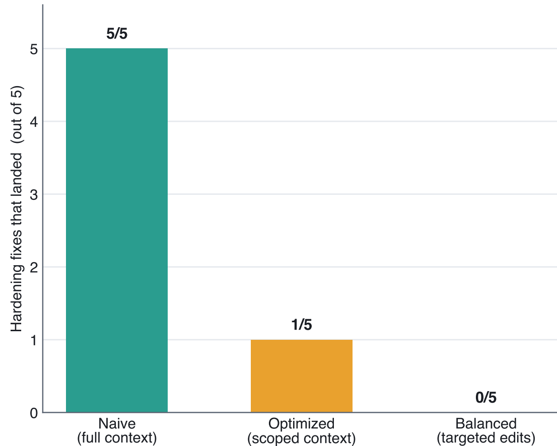
...but correctness collapses
