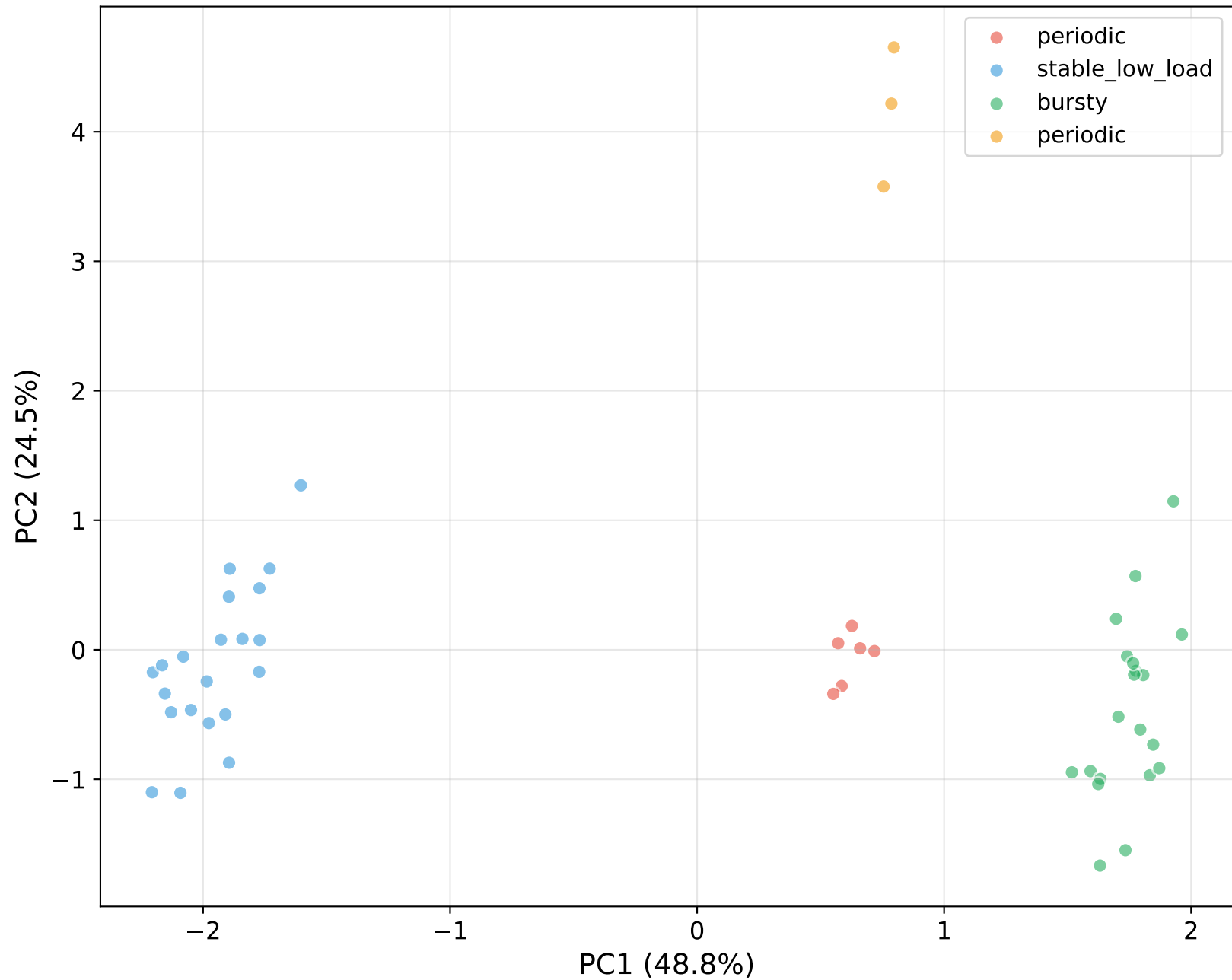
Workload Pattern Clusters (PCA Visualization)
