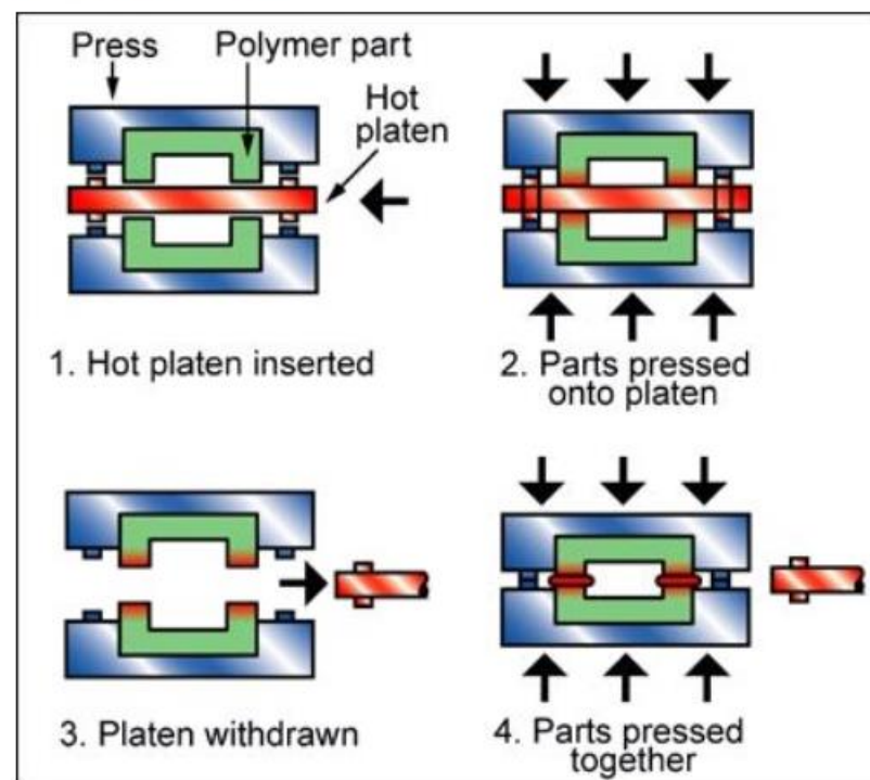
Process schematic
