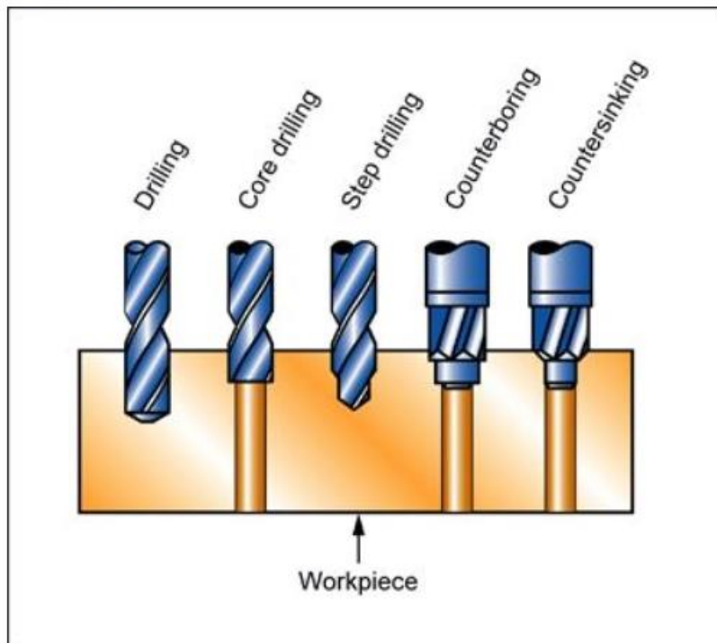
Process schematic
