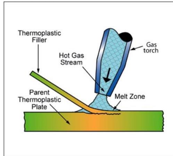
Process schematic
