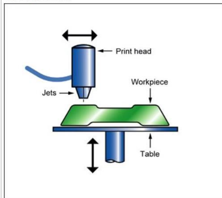
Process schematic
