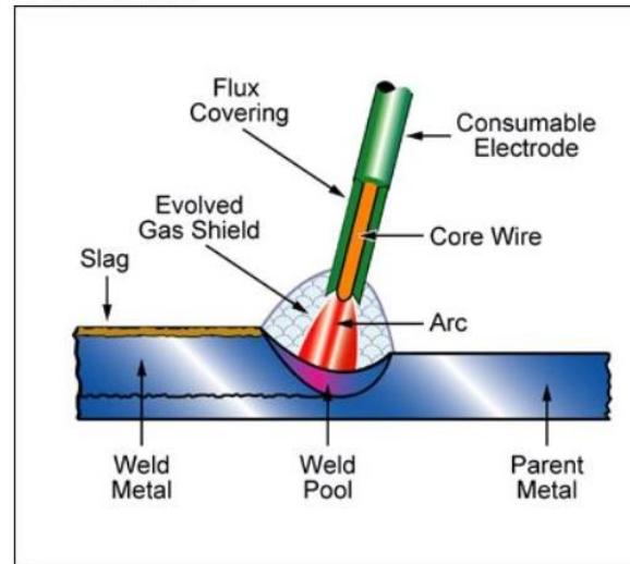
Process schematic
