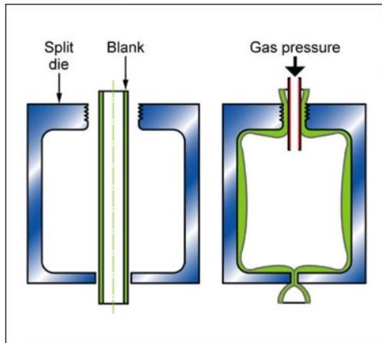
Process schematic
