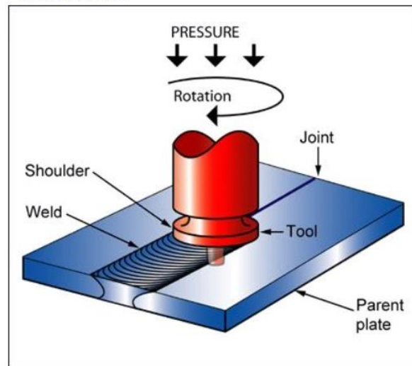
Process schematic
