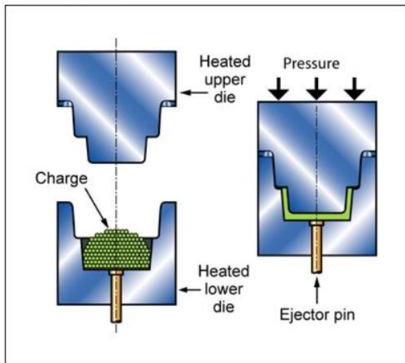
Process schematic
