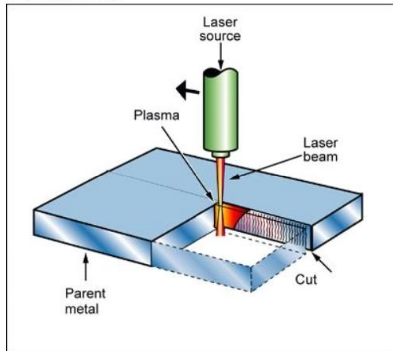
Process schematic
