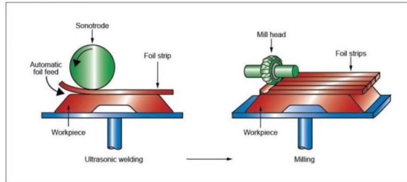
Process schematic
