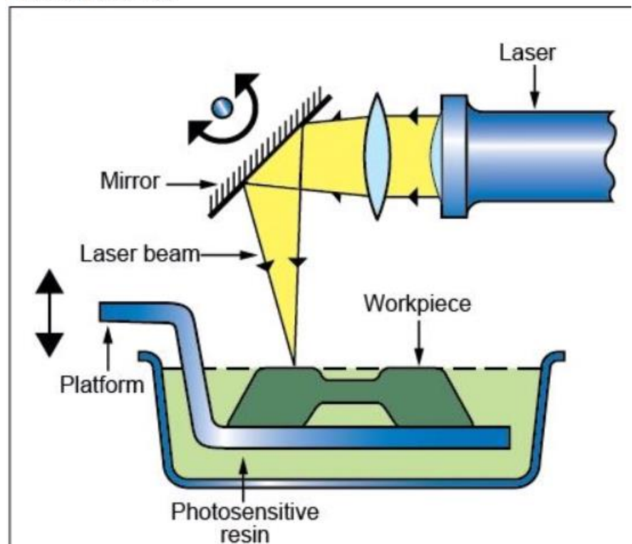
Process schematic
