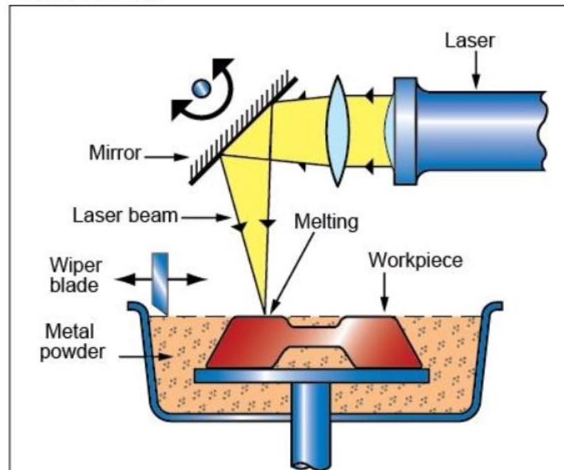
Process schematic
