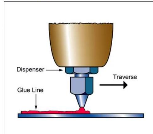
Process schematic
