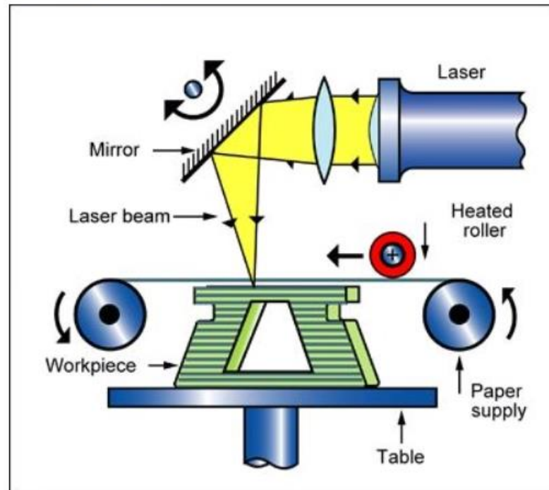
Process schematic
