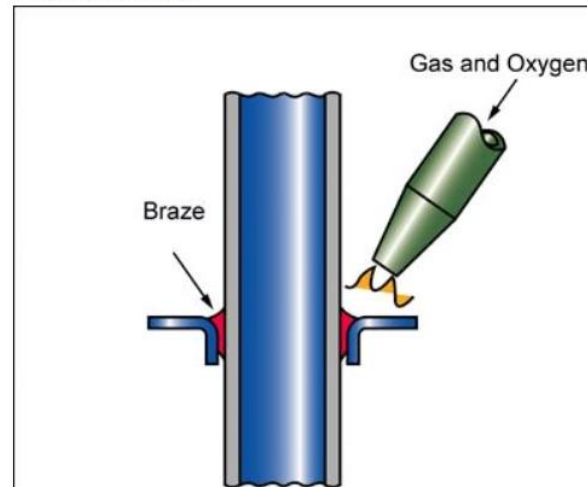
Process schematic
