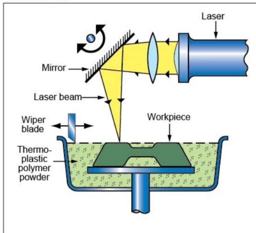
Process schematic
