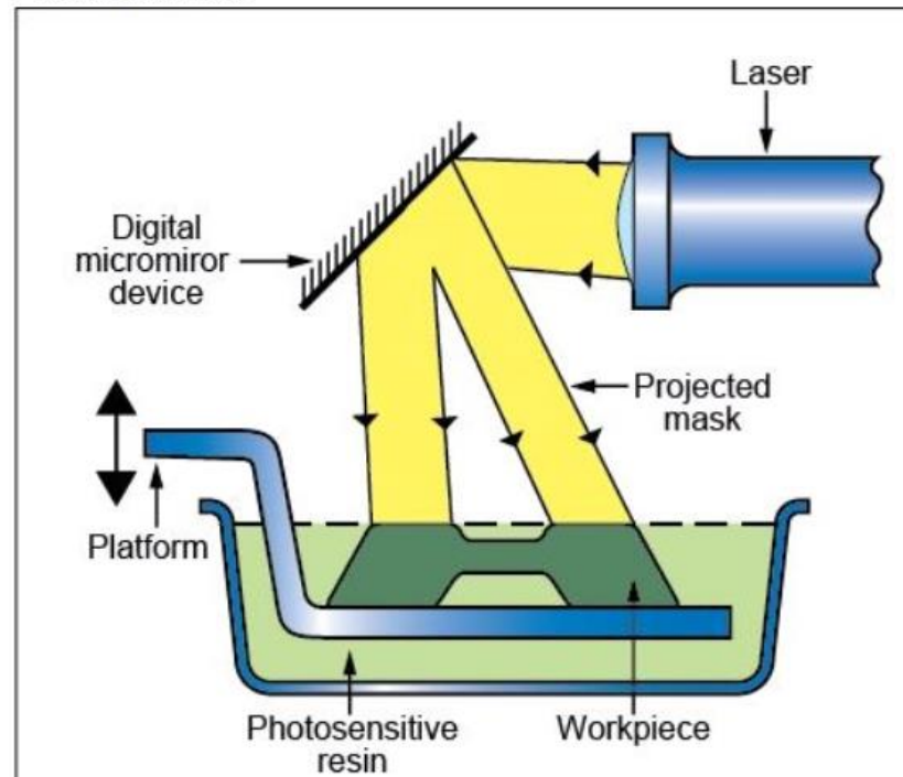
Process schematic
