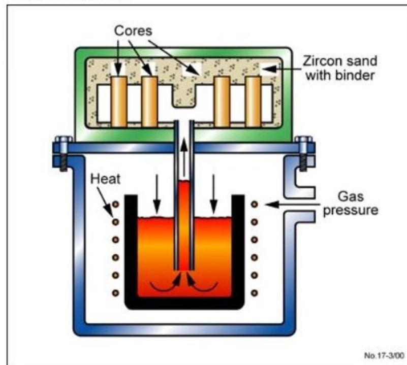
Process schematic
