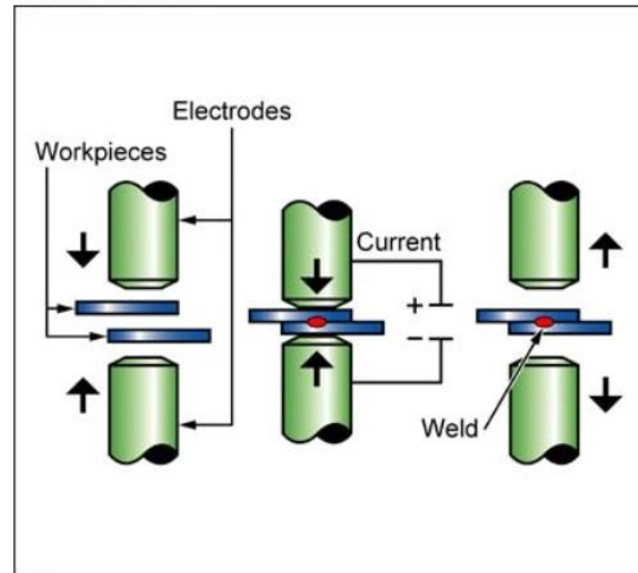
Process schematic
