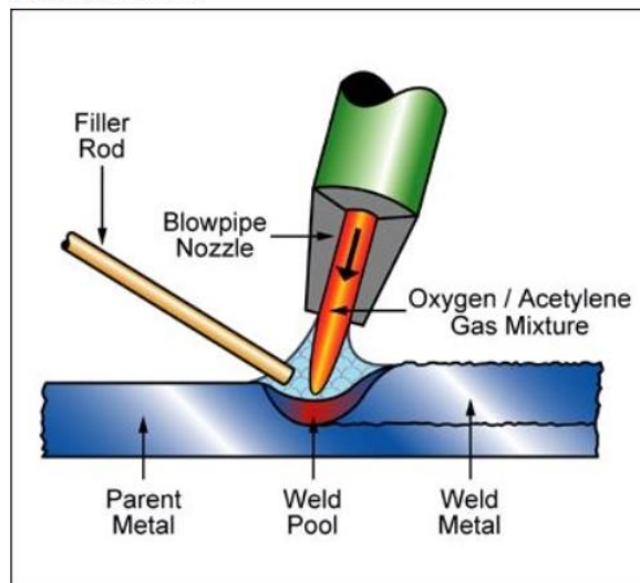
Process schematic
