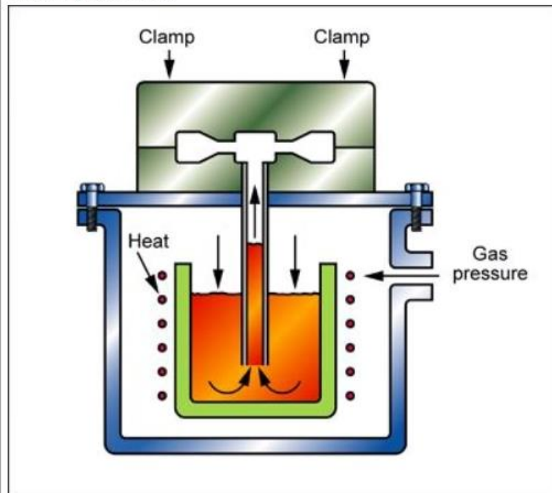
Process schematic
