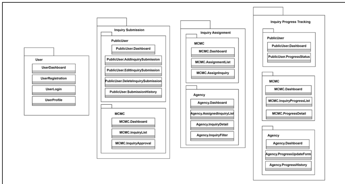
Figure 3.1 Application Layer for MySebenarnya Systems
