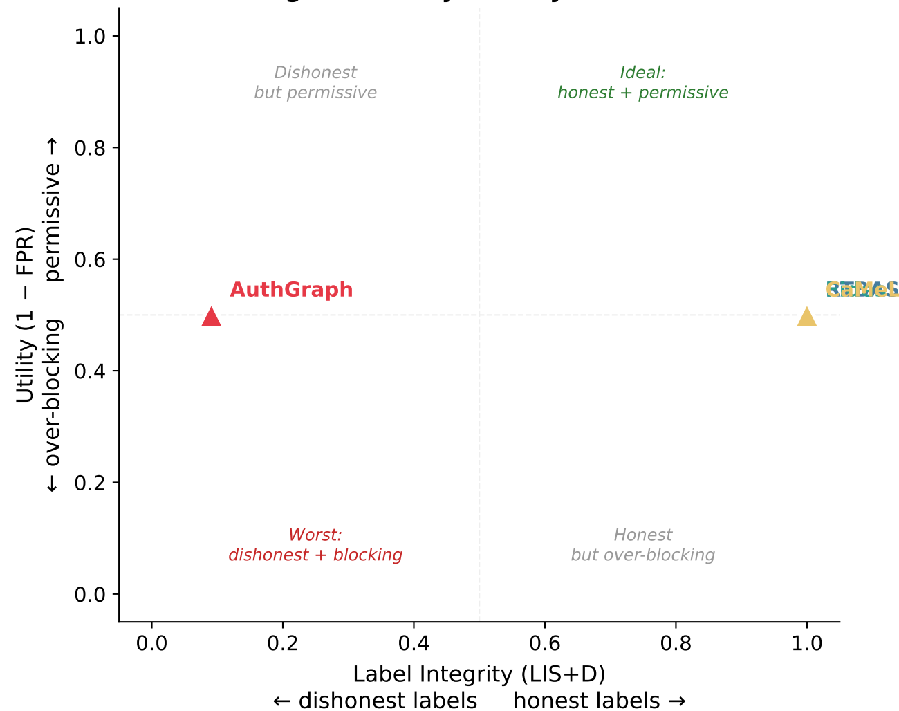
Fig 3: Security / Utility Trade-Off
