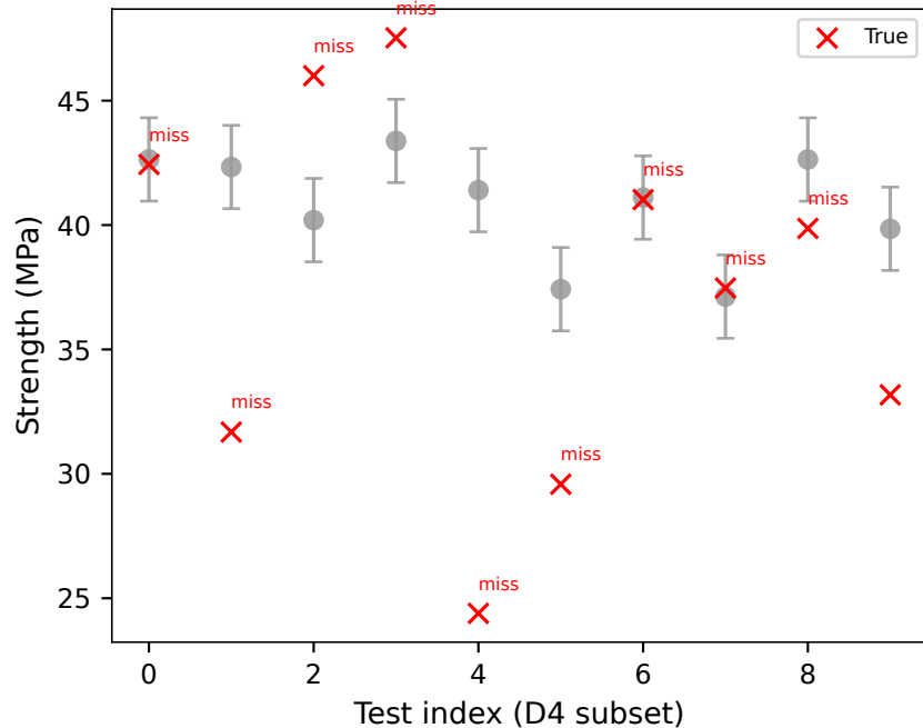
SplitCP (source-calibrated) cov=5%, width=3.3 MPa
