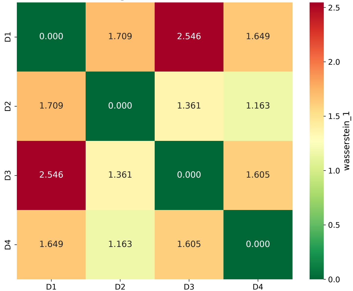
Distribution Shift: wasserstein_1 (Higher = More Shift)
