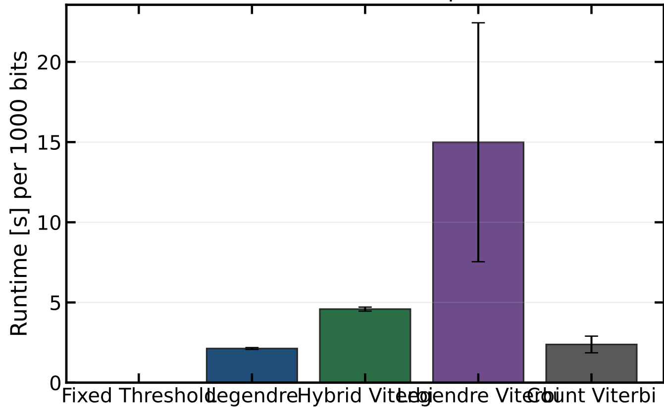
Detector runtime comparison
