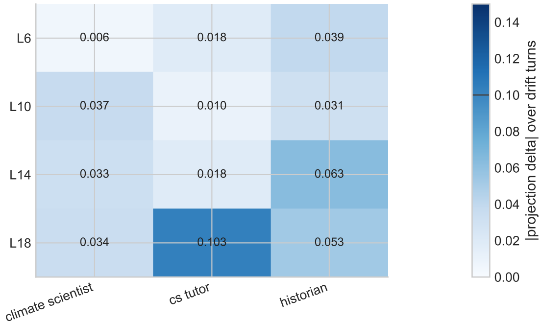
llama3.1-8b-instruct
