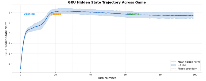
Figure 4: Hidden state norm across turns (mean \pm std over 200 games). The charge-stabilize-decay pattern is consistent across all games.
