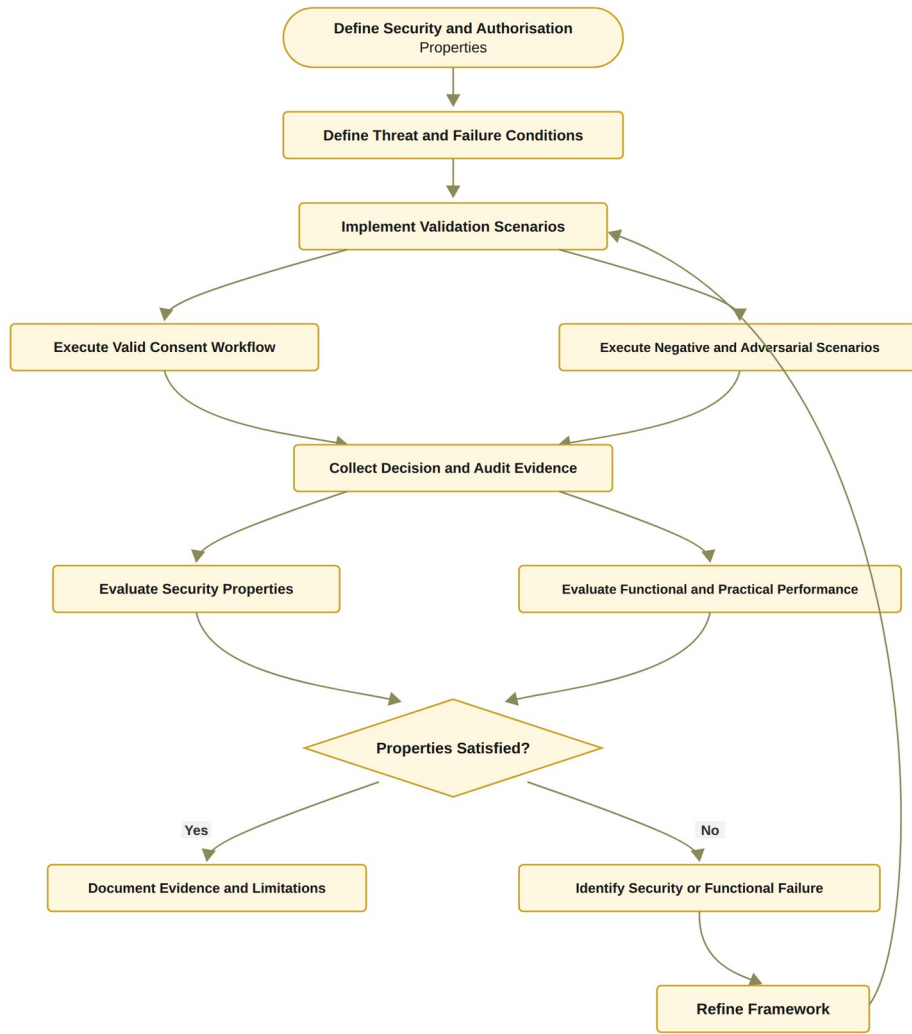
Figure 12: RO6 workflow for formal security assurance and empirical validation
