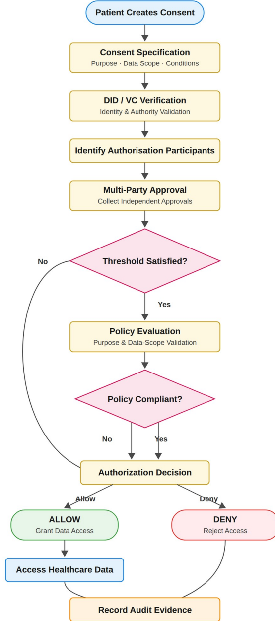
Figure 6: End-to-End Workflow of Trust-Oriented Consent Authorisation Framework
