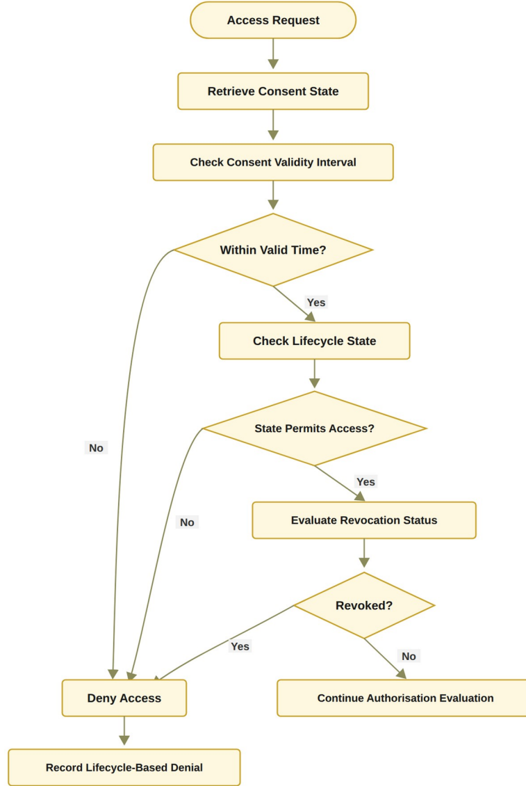
Figure 14: RO5 workflow for temporal and consent lifecycle trust
