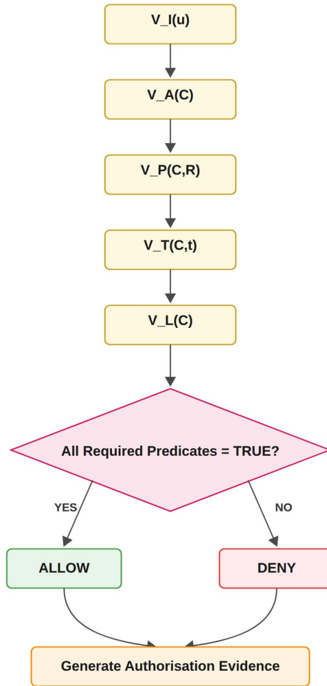
Figure 8: Trust Predicate Evaluation and Authorisation Decision Flow
