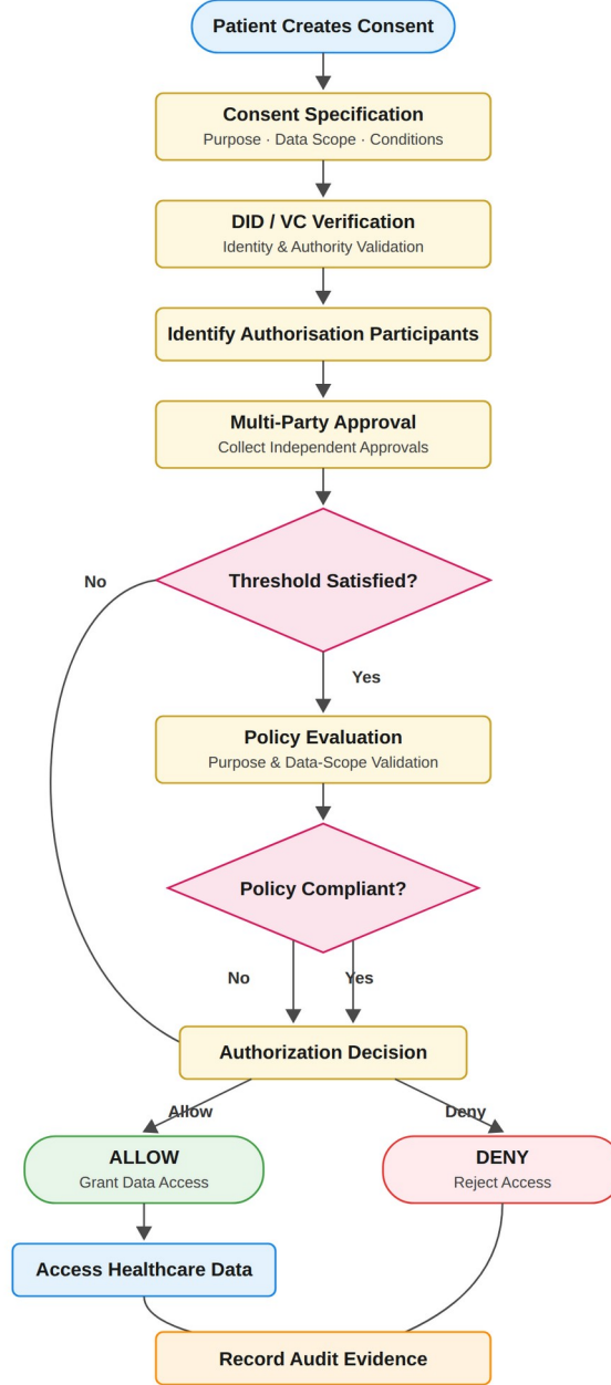
Figure 9: End-to-end workflow of the trust-oriented consent authorisation framework
