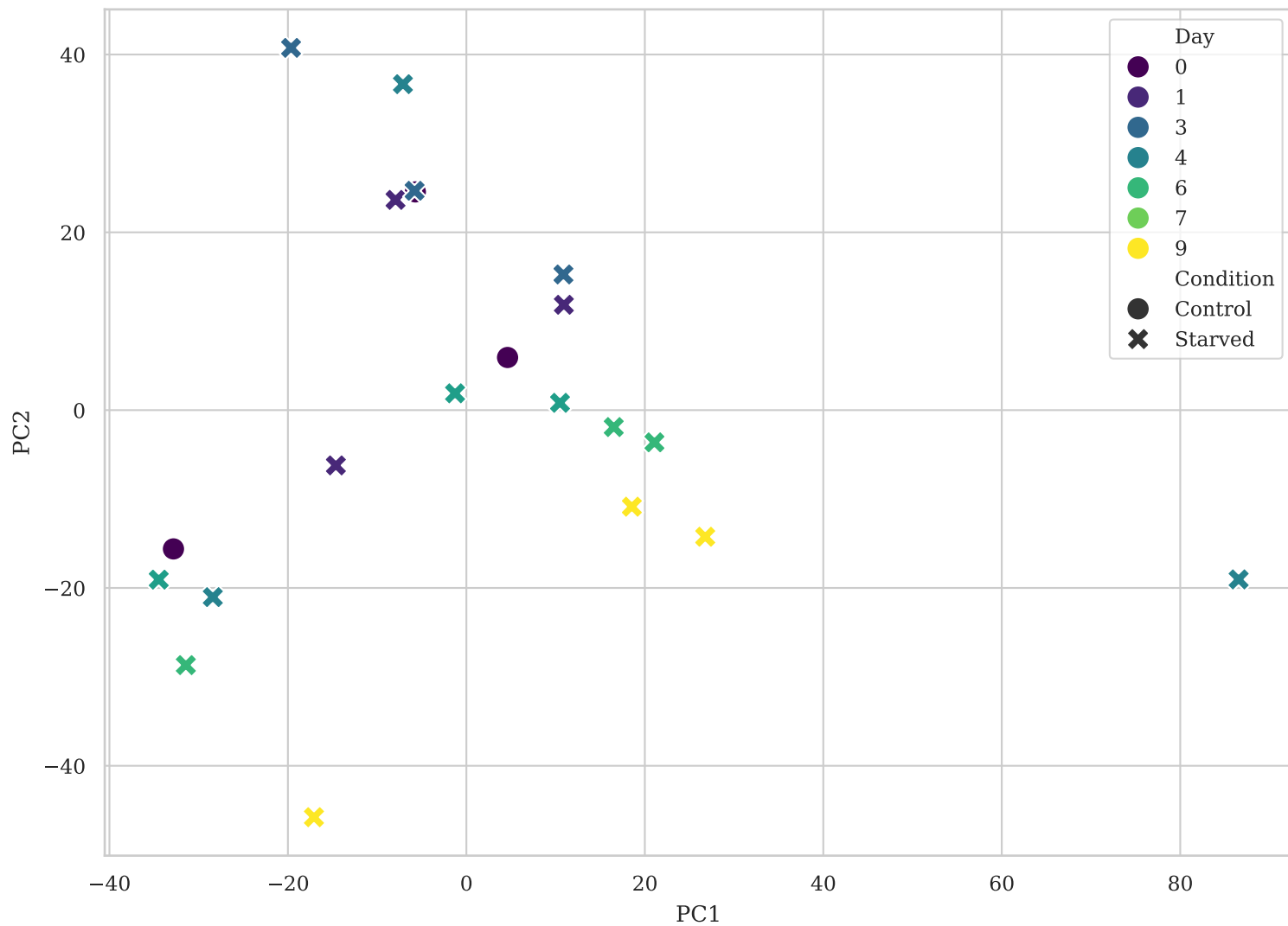
PCA of GSE129964 (Serum Starvation Timecourse)
