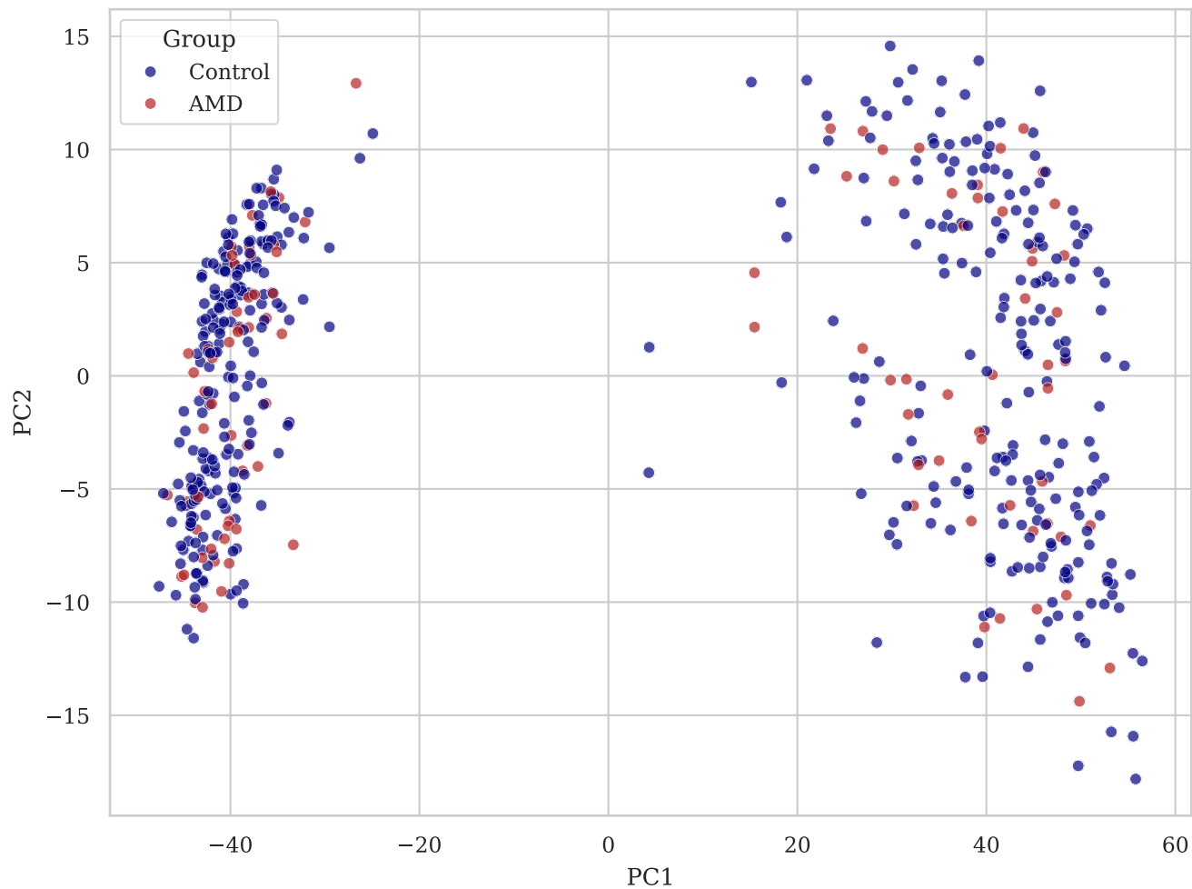
PCA of GSE135092 (Top 2000 Genes) Explained Var: 83.8% / 2.2%
