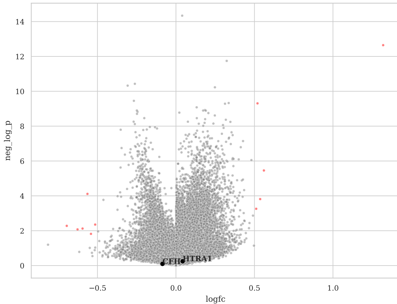
Volcano Plot: AMD vs Control
