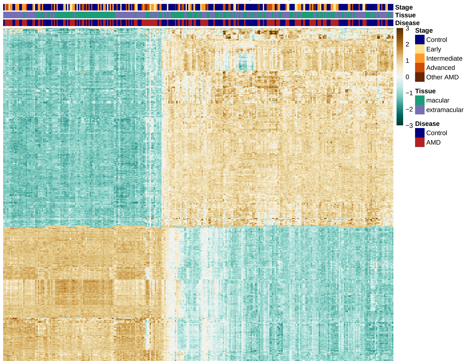
GSE29801: Top 500 Variable Genes (Z-scored)
