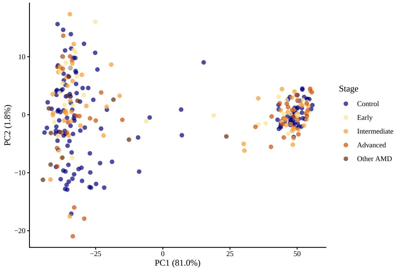
GSE29801: PCA by AMD Staging
