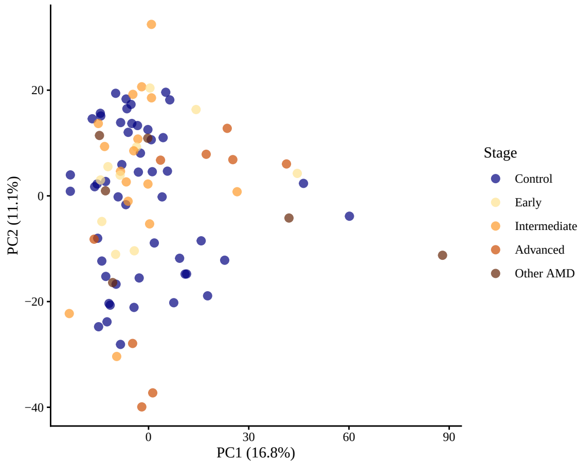
macular RPE-choroid: PCA by Staging
