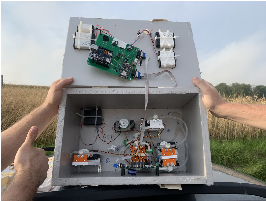
Fig. 3: Experiment assembly post launch.
