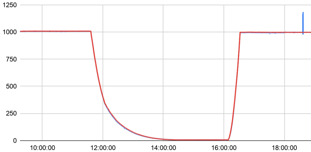
Fig. 9: Pressure readings [hPa].
