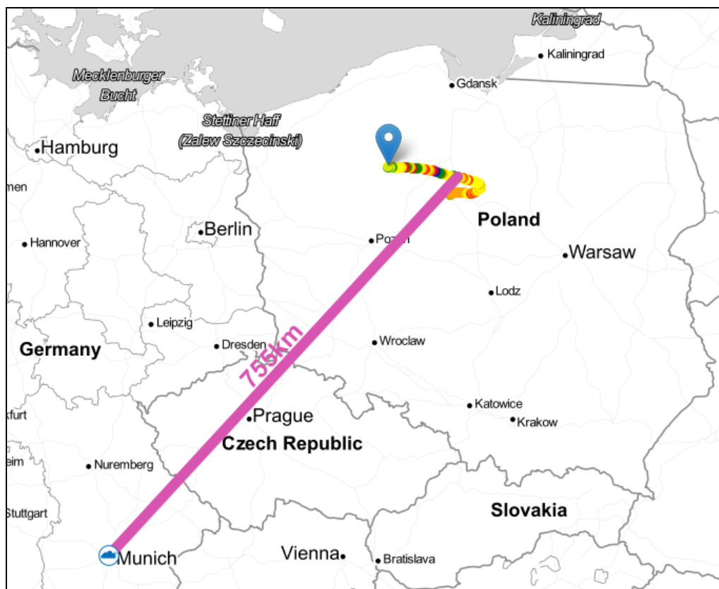
Fig. 5: Ground path and the longest packet acquisition line of sight.
