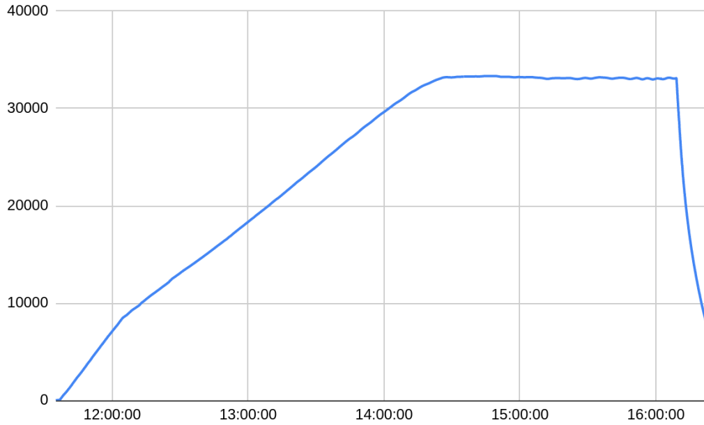
Fig. 7: GPS based flight profile [m]
