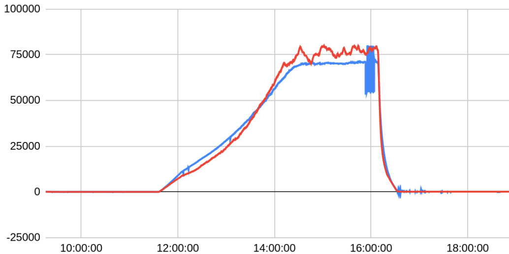
Fig. 8: Pressure and temperature based altitude calculation [m].
