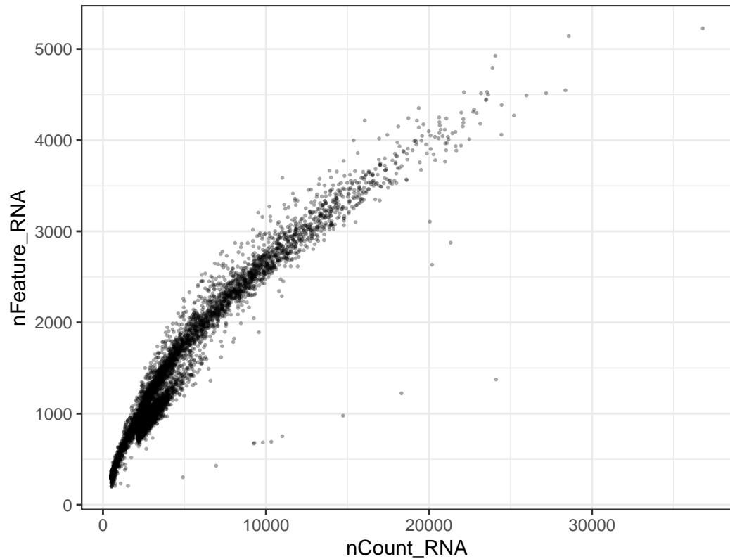
nCount vs nFeature – IA_1
