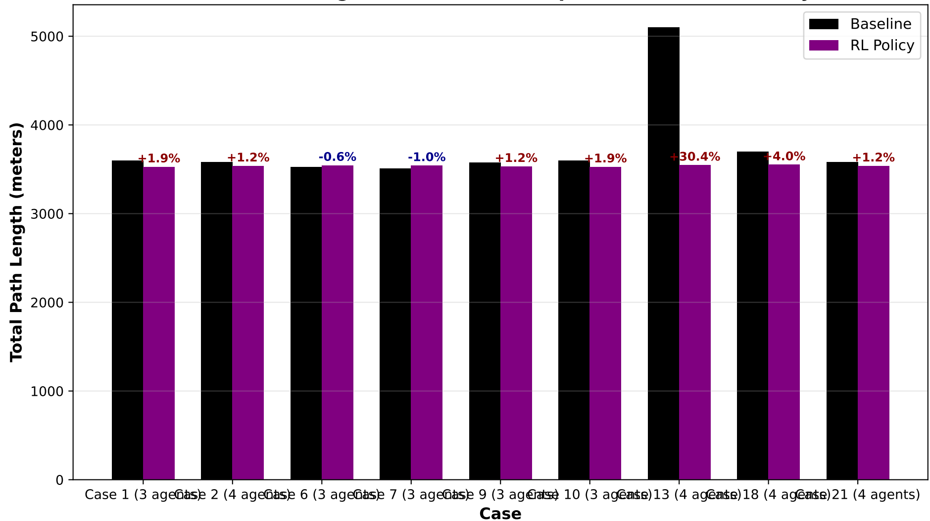
Total Path Length Traveled (Ownship): Baseline vs RL Policy
