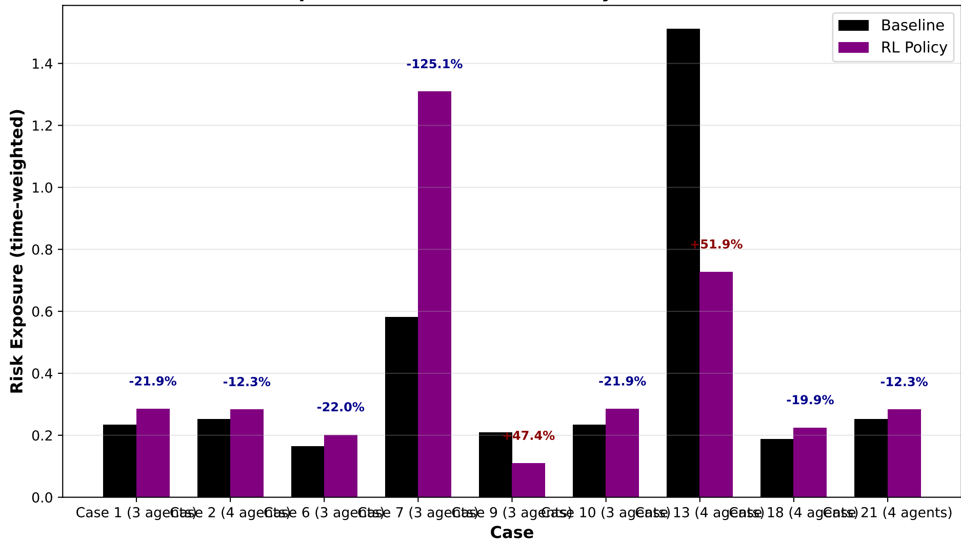
Risk Exposure: Baseline vs RL Policy (Lower is Better)
