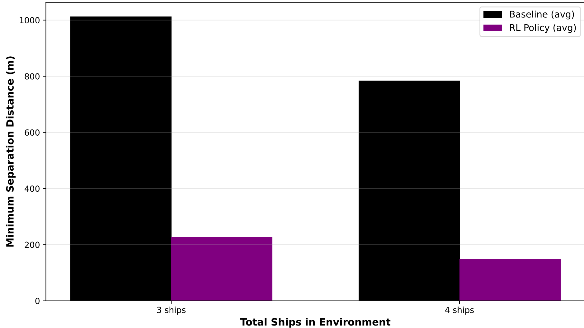
Minimum Separation Distance Scaling: Impact of Ships in Environment
