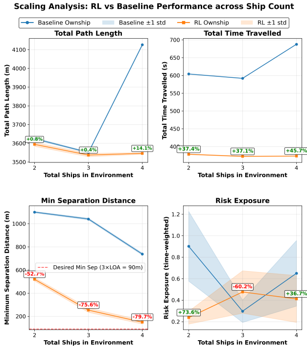
Fig. 2. Aggregate performance trends between RL-based and rule-based ownship planners across increasing number of agents 2–4 vessel scenarios evaluated over 50 simulations each
