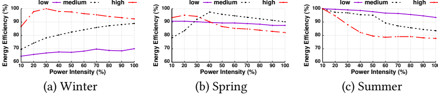
Fig. 11. Energy-efficiency across three seasons: (a) winter, (b) spring, and (c) summer. For each season, we evaluate our three designs that are winter-optimal (red line, long dash), spring-optimal (black line, small dash), and summer-optimal (purple line, solid) over various operating points represented by power intensity of x-axis.
