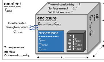
Fig. 6. A simple thermodynamic model of environmentally-powered computer systems.
