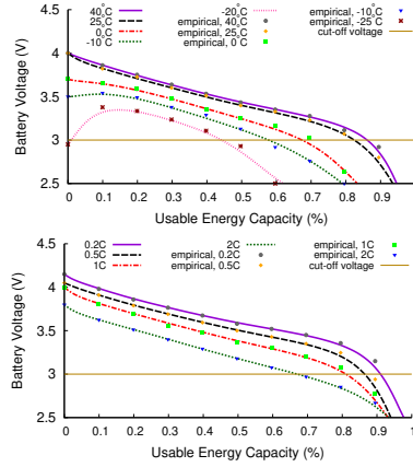
Fig. 2. Usable battery capacity varies with temperature (top) and discharge current (bottom).
