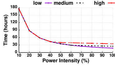
Fig. 13. Performance during summer for high (winter-optimal), medium (spring-optimal), and low (summer-optimal) insulation designs over various operating points.
