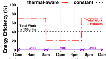
Fig. 9. Work done using a naive and thermal-aware scheduling approach that exploits the feedback loop between electrical and thermal energy.
