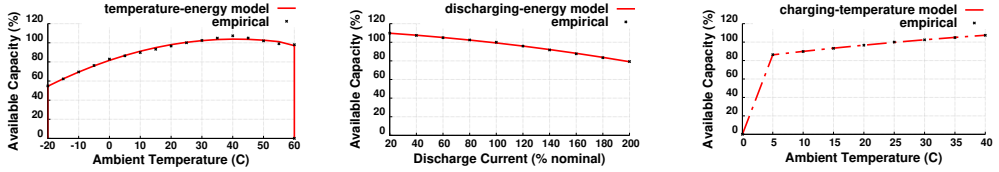
(a) Temperature-Energy Effect (b) Discharge-Energy Effect (c) Temperature-Charging Effect
