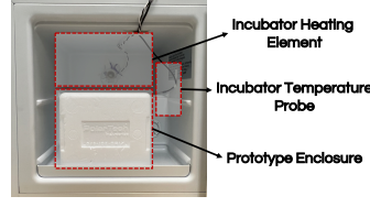
Fig. 8. Small-scale prototype inside the incubator.
