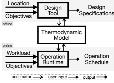
Fig. 5. An overview of Acclimator including its key modules, input requirements, and output parameters.
