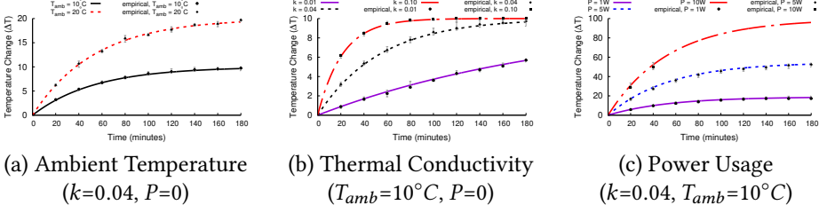
Fig. 7. The change in the enclosure's temperature T_{enc} over time is a function of the (a) ambient temperature T_{amb} , (b) the enclosure's thermal conductivity k , and (c) the processor's power usage P .
