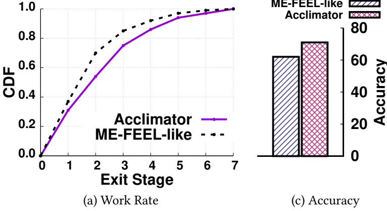
Fig. 15. Performance comparison against a modified MultiExit Federated Edge Learning (ME-FEEL) approach [24]. Acclimator outperforms ME-FEEL by exiting in a higher stage leading to a higher accuracy of the trained model.
