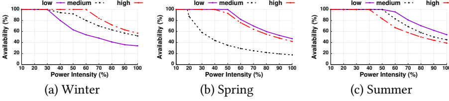
Fig. 12. Availability across three seasons: (a) winter, (b) spring, and (c) summer. For each season, we evaluate our three designs that are winter-optimal (red line, long dash), spring-optimal (black line, small dash), and summer-optimal (purple line, solid) over various operating points represented by power intensity of x-axis.
