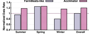
Fig. 14. Performance comparison against Farmbeats. Acclimator outperforms Farmbeats thermal-agnostic design during the summer and winter months. Both have the same performance during spring season.
