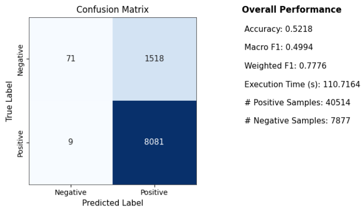
LABR_Preprocessed with AdaBoostClassifier
