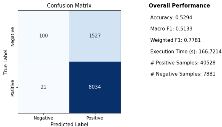
LABR with AdaBoostClassifier
