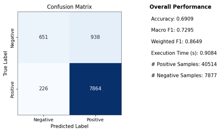
LABR_Preprocessed with LinearSVC
