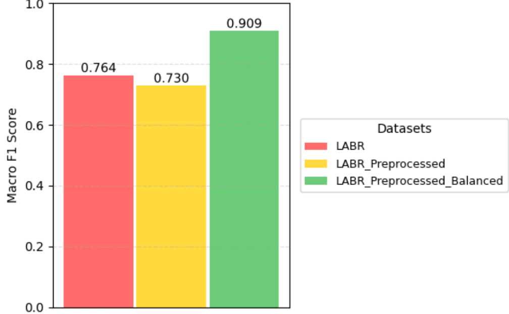
Macro F1 Score by Dataset (LinearSVC)
