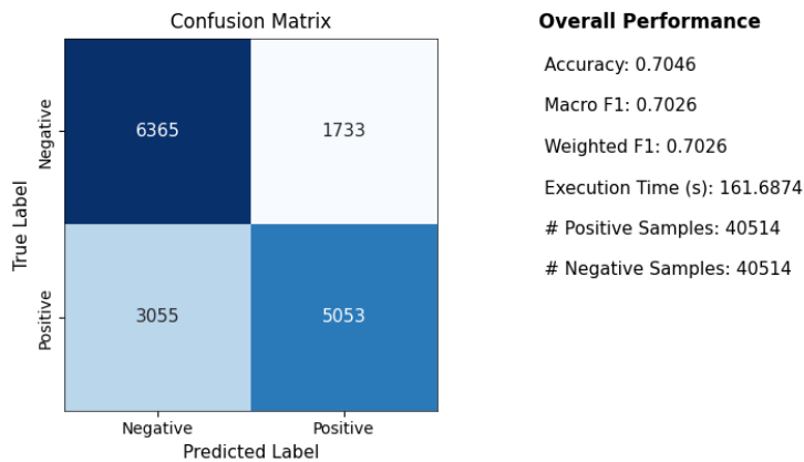
LABR_Preprocessed_Balanced with AdaBoostClassifier
