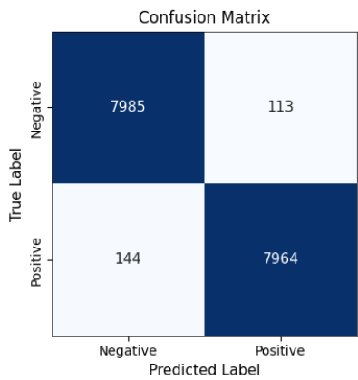
LABR_Preprocessed_Balanced with RandomForestClassifier
