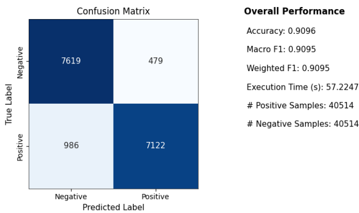
LABR_Preprocessed_Balanced with LinearSVC
