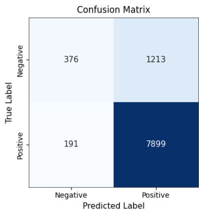
LABR_Preprocessed with RandomForestClassifier
