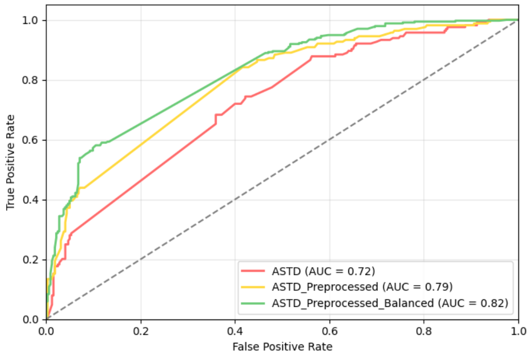
ROC Curves - AdaBoostClassifier
