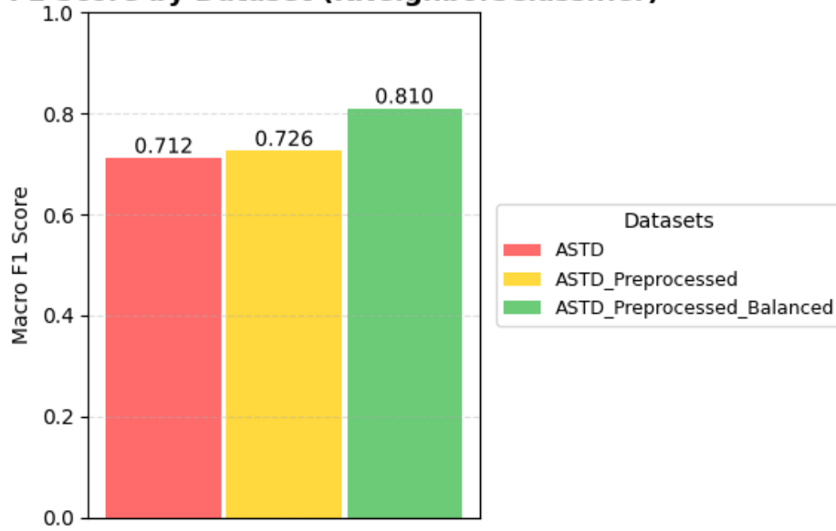
Macro F1 Score by Dataset (KNeighborsClassifier)
