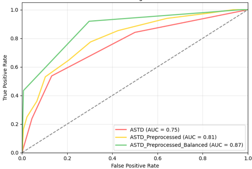
ROC Curves - KNeighborsClassifier
