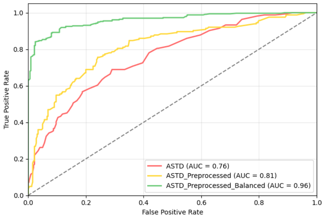
ROC Curves - RandomForestClassifier
