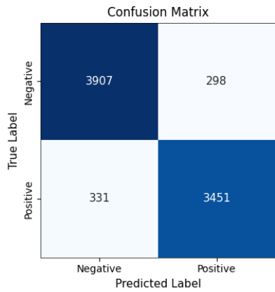
TESA_Preprocessed with LinearSVC
