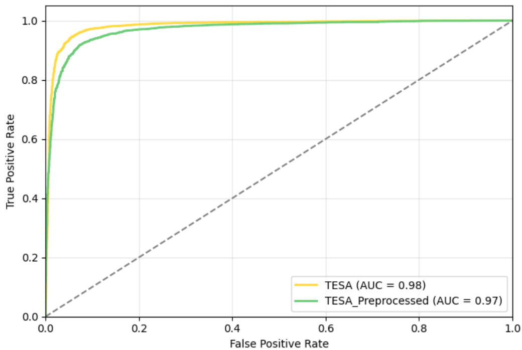
ROC Curves - LinearSVC
