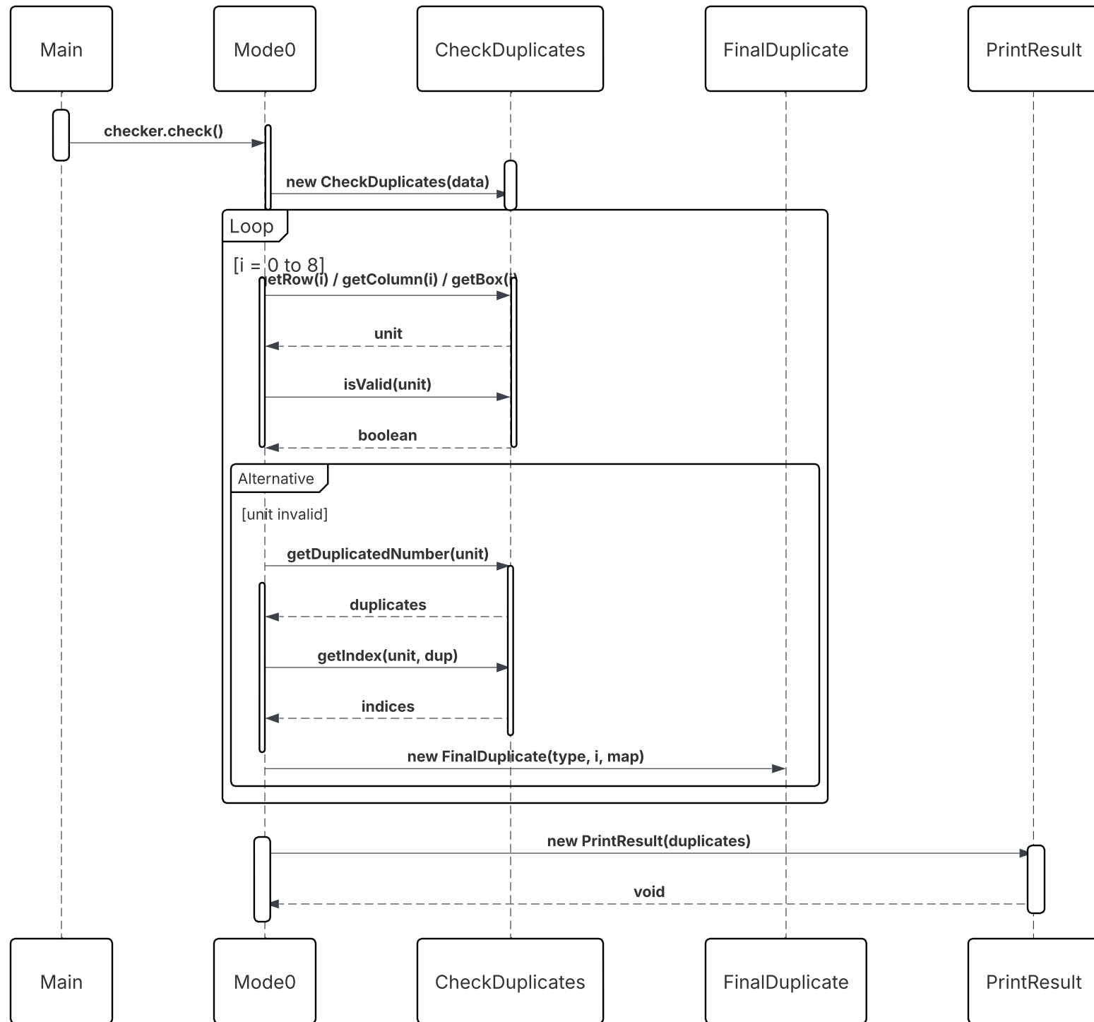
Mode0 Sequence Diagram
