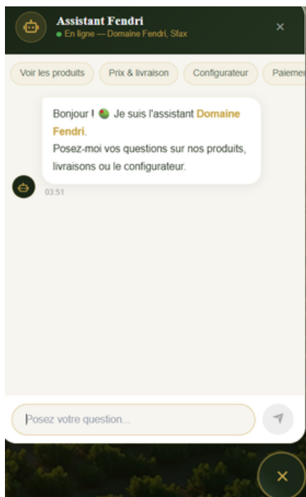
Figure 63 : Agent chatbot
