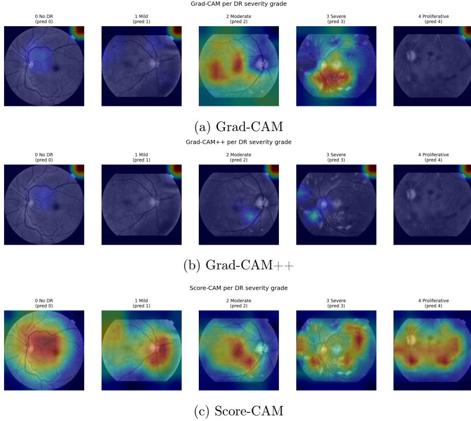
Figure 5: Qualitative explainability comparison for the selected EfficientNetB3 model. Heatmaps are useful for auditing, but corner and border activations prevent lesion-level claims.
