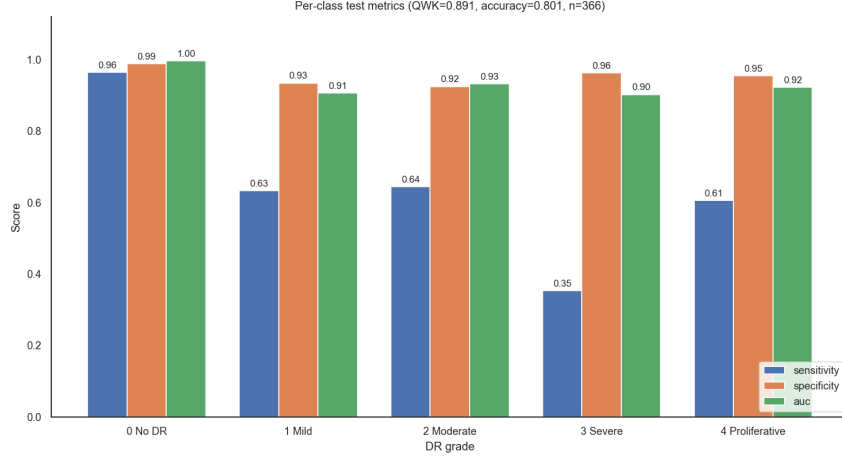
Figure 3: Per-class sensitivity, specificity, and one-vs-rest AUC for the selected EfficientNetB3 model.
