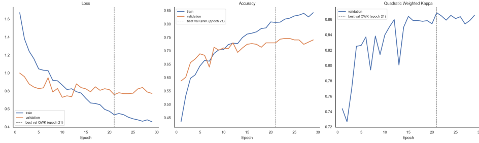
Figure 4: EfficientNetB3 training curves reconstructed from the MLflow metric history. The best validation-QWK checkpoint is selected for held-out test evaluation.
