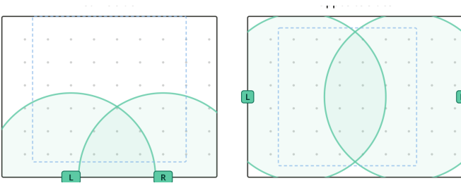
Fig. 2. Arm-mounting geometry trade-off. Left: centered arms with overlapping reach envelopes concentrated near the bases. Right: separated outer-edge layout with the fold zone centered between the arms (selected). The dashed rectangle marks the workspace; shaded regions are per-arm reach.
