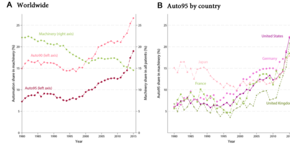
FIG. 2.—Share of automation patents in machinery and share of machinery patents for biadic families. A , Share of auto95 and auto90 patents in machinery (left axis) and share of machinery patents in all patents (right axis) worldwide. B , Share of auto95 patents in machinery by applicants' nationality. Patents with multiple C/IPC codes are counted only once.
