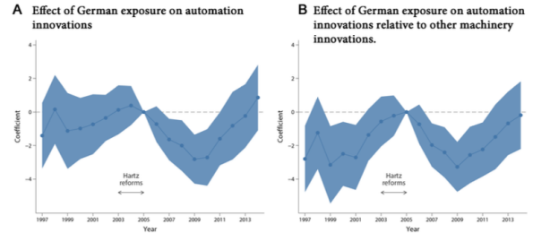
FIG. 5.—Effect of German exposure on automation innovations. A reports coefficients on the interaction between the German weight and a set of year fixed effects in a Poisson regression of auto95 innovations controlling for a full set of fixed effects and firm innovation stocks with 2,156 firms. B reports coefficients on the triple interaction between the German weight, a dummy for auto95 innovations, and a set of year fixed effects in a regression of auto95 and other machinery innovations controlling for a full set of fixed effects, firm innovation stocks, and the interaction between the German weight and a set of year fixed effects with 6,692 firms. Standard errors are clustered at the firm level, and the shaded areas represent 95% confidence intervals. The figure shows that the relative trend in automation innovation for firms more exposed to Germany reversed after the Hartz reforms.
