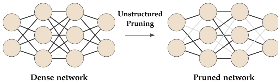
Figure 2.2: Illustration of unstructured pruning. The architecture is unchanged, but individual weights are removed independently.
