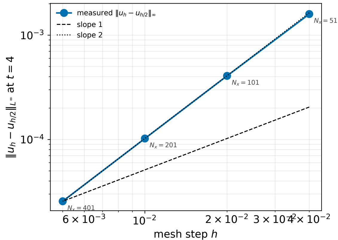
(a) mesh refinement, \Delta t = 2.5 \cdot 10^{-3}
