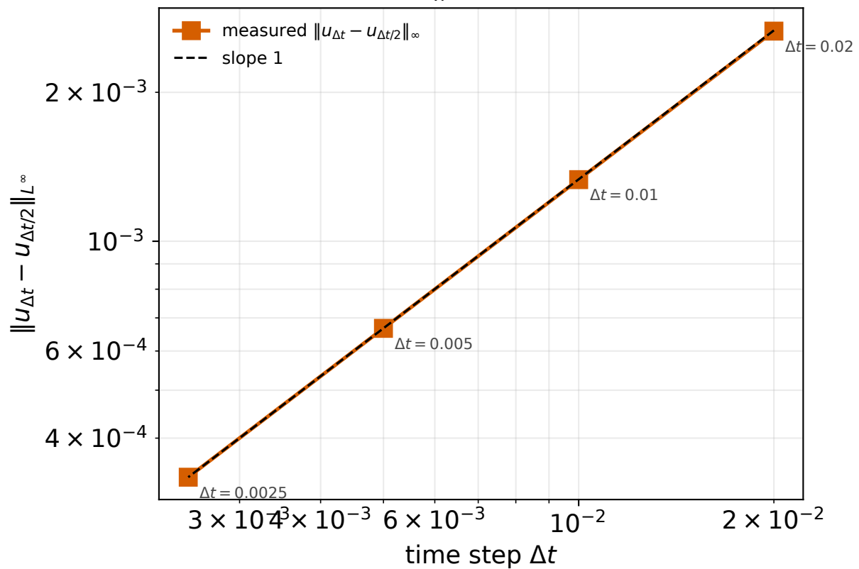
(b) time refinement, N_x = 101
