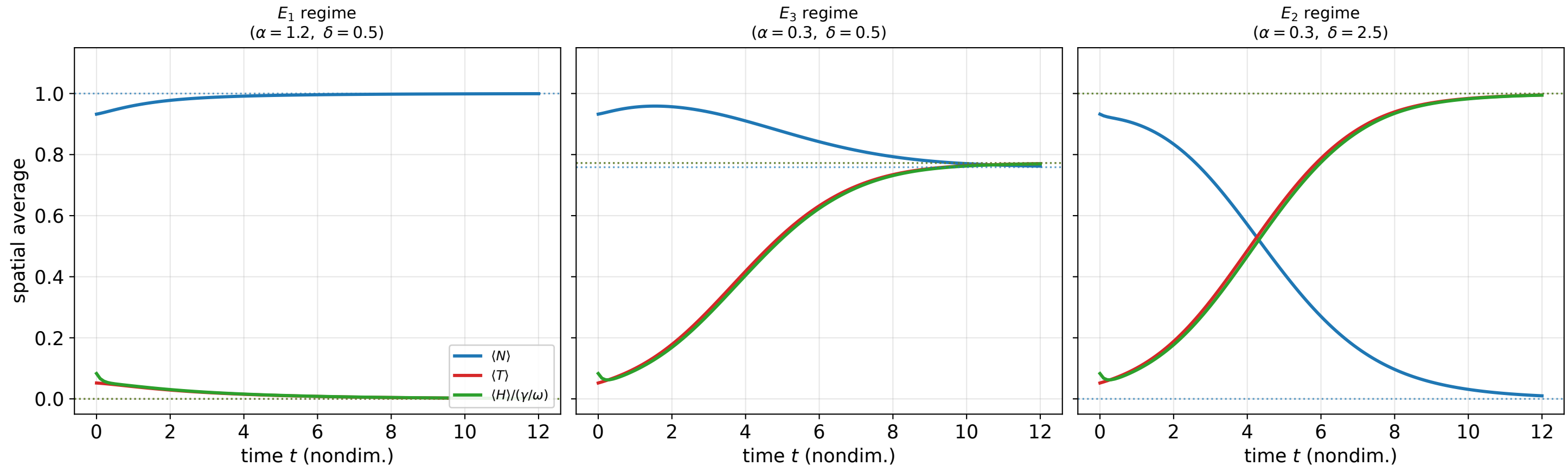
Macroscopic observables \langle N \rangle, \langle T \rangle, \langle H \rangle / (\gamma/\omega) vs time. Dotted lines: predicted equilibrium values.
