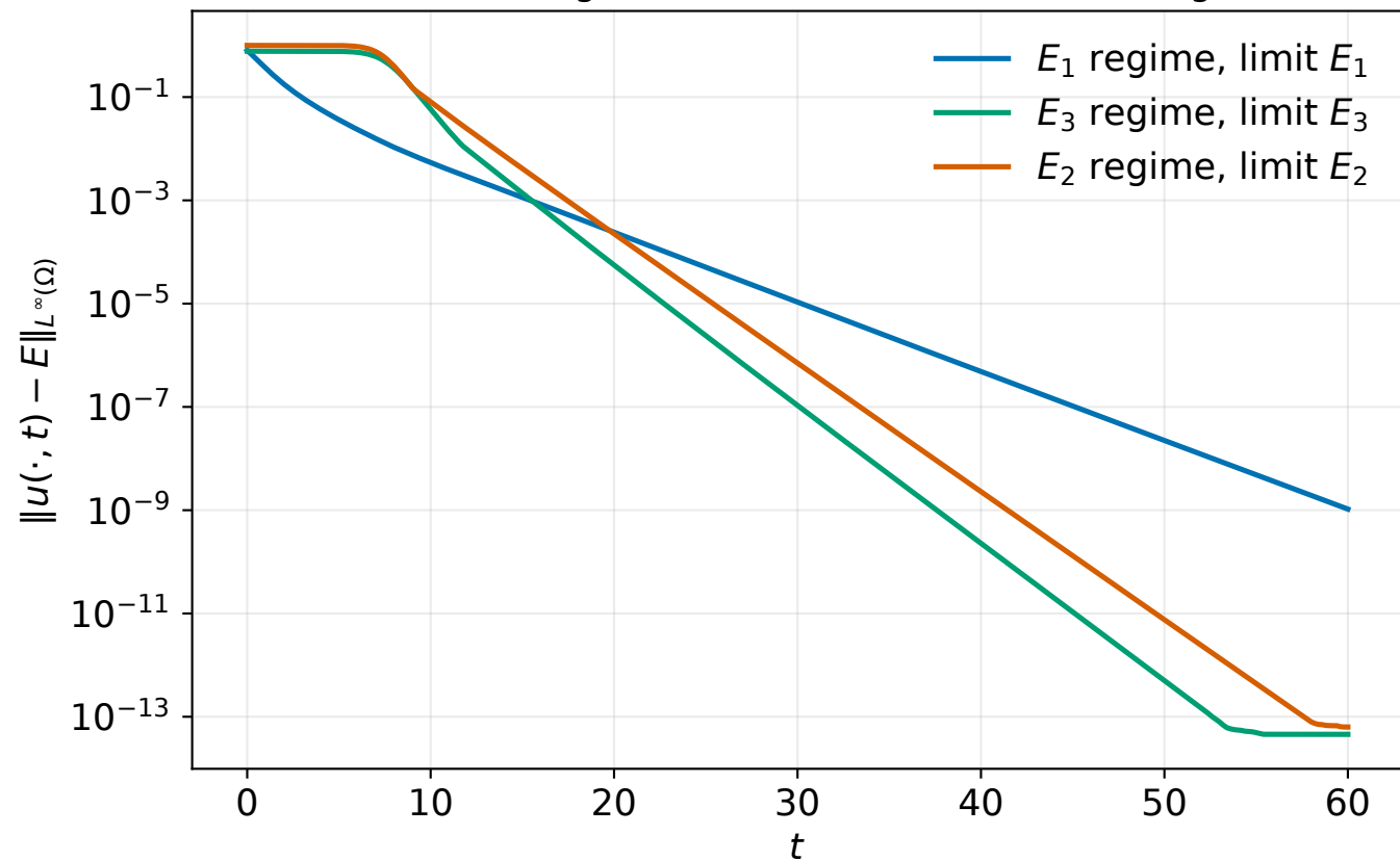
Uniform convergence in the three non-bistable regimes
