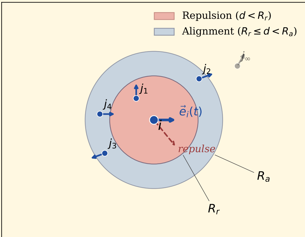
(a) Two-zone Vicsek update (full 360° vision)
