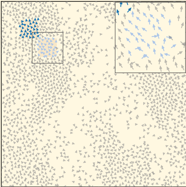
motility adaptive \eta = 0.1, \langle \varphi \rangle = 0.52, n_{cl} = 2
