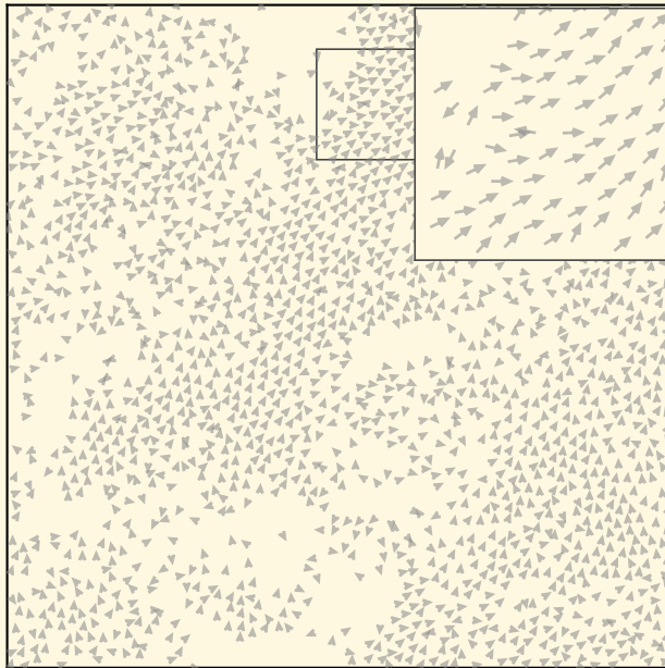
double-adaptive \eta = 0.1, \langle \varphi \rangle = 0.66, n_{cl} = 0
