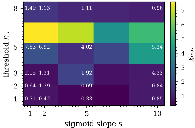
(a) \chi_{\max} (full mode, L = 22 )
