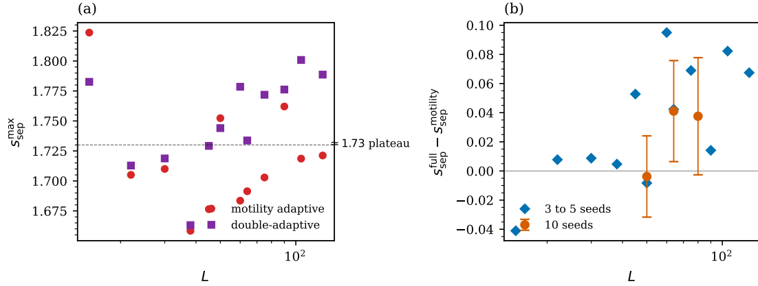
Figure 7. Combined twelve-size scan of the density-separation index. Panel (a): s_{\text{sep}}^{\text{max}} versus L for the motility-only ablation (orange) and the double-adaptive model (purple), built by combining the seven-size controlled FSS (three seeds) with a fine-grid five-size scan (five seeds, L \in \{38, 50, 60, 75, 105\} ). Panel (b): the gap s_{\text{sep}}^{\text{full}}(L) - s_{\text{sep}}^{\text{motility}}(L) on the same horizontal axis.
