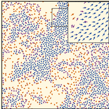
Near-critical \eta = 0.1, \langle \phi \rangle = 0.66
