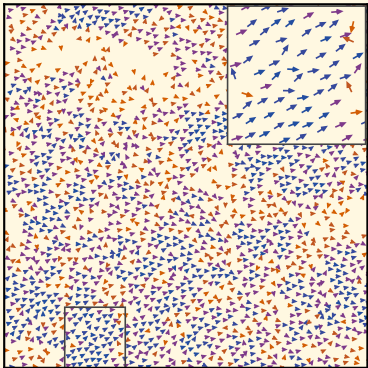
Ordered \eta = 0.02, \langle \phi \rangle = 0.79
