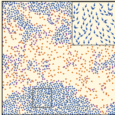
Disordered \eta = 0.3, \langle \phi \rangle = 0.39
