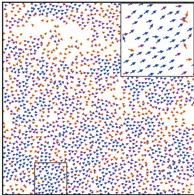
(a) Ordered \eta = 0.02 , \langle \varphi \rangle = 0.79
