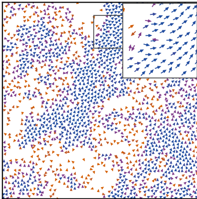
(b) Near-critical \eta = 0.1 , \langle \varphi \rangle = 0.66
