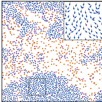
(c) Disordered \eta = 0.3 , \langle \varphi \rangle = 0.39
