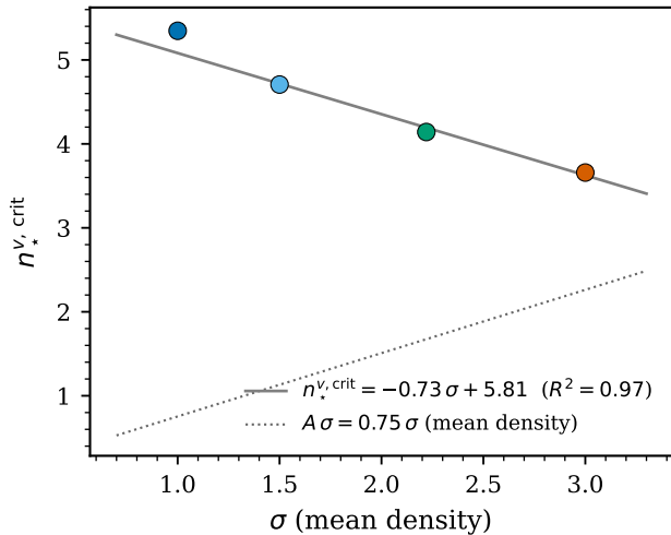
(b) Linear scaling test, weighted fit
