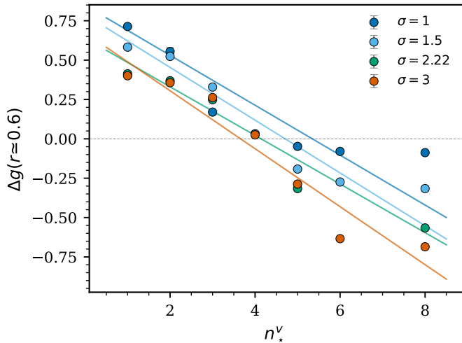
(a) \Delta g(n_\star^v) at four densities
