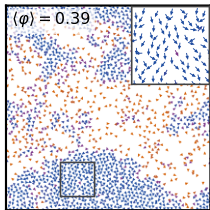
double-adaptive
