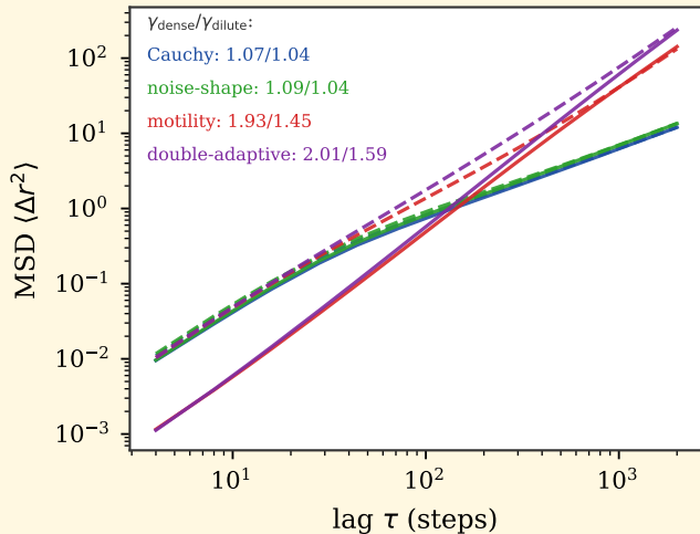
(b) stratified MSD
