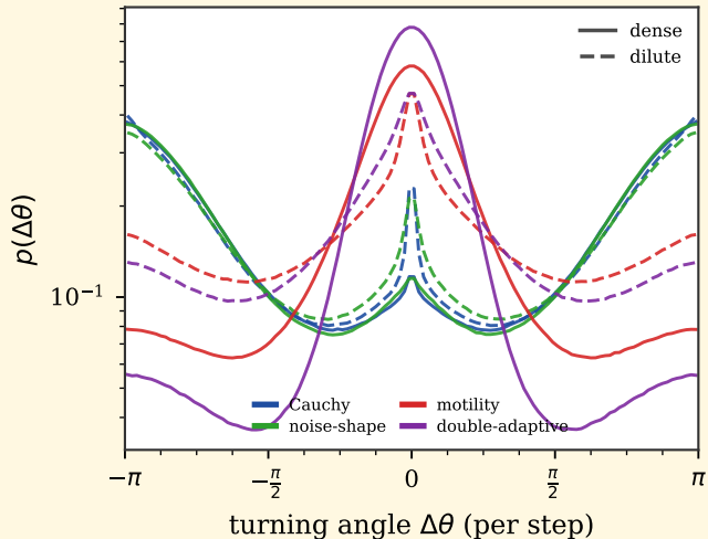
(a) turning-angle pdf
