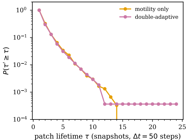
(a) Patch-lifetime survival, L = 30 , 10 seeds
