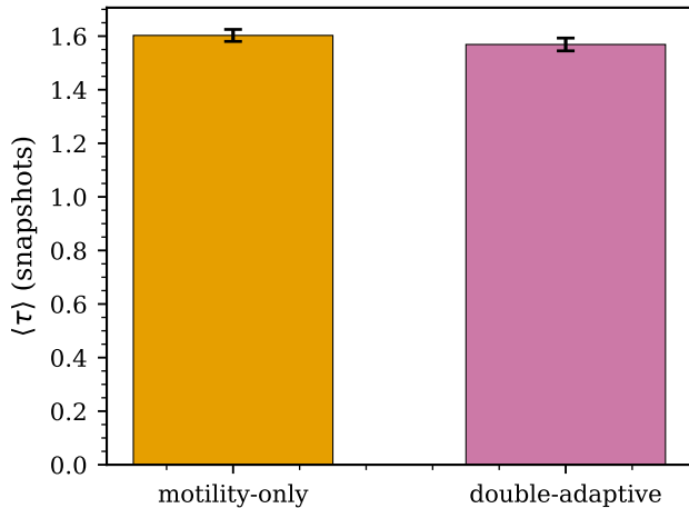
(b) Mean patch lifetime, aggregated
